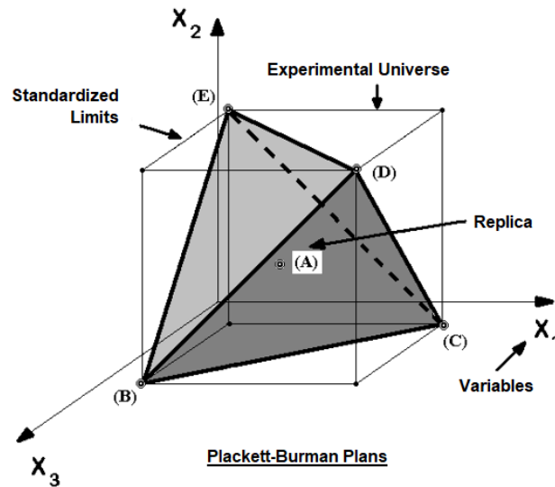
Figure 1. Plackett-Burman plans. Orthogonal “half-factorial” arrangement.
