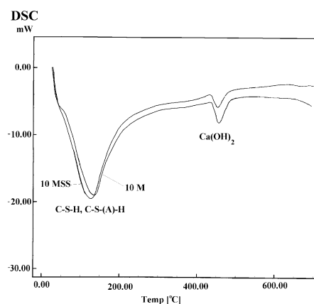
Figure 13. DSC curves for 10M and 10MSS pastes.
