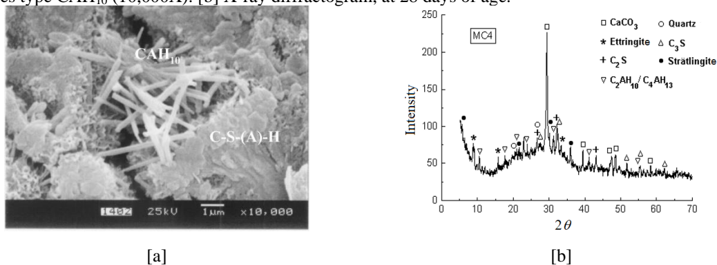
Figure 7. [a] Micrograph (SEM) of the paste with 50% MK and 15% Na_2O (MC4) at 7 days of age. Detail of the formation of aluminate phases type CAH_{10} (10,000X). [b] X-ray diffractogram, at 28 days of age.
