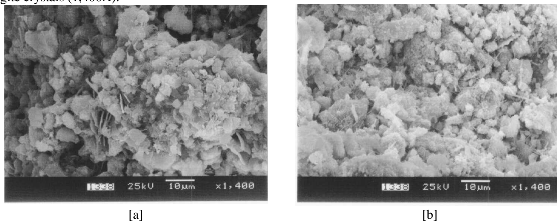
Figure 15. Micrographs (SEM) of the pastes containing: [a] 50% MK and 5% \text{Na}_2\text{SiO}_3 (50MSS). Porous microstructure formed by large particleboard (1,400X); [b] 70% MK (70M). Microstructure formed by the agglutination of partially dissolved particles and ettringite crystals (1,400X).
