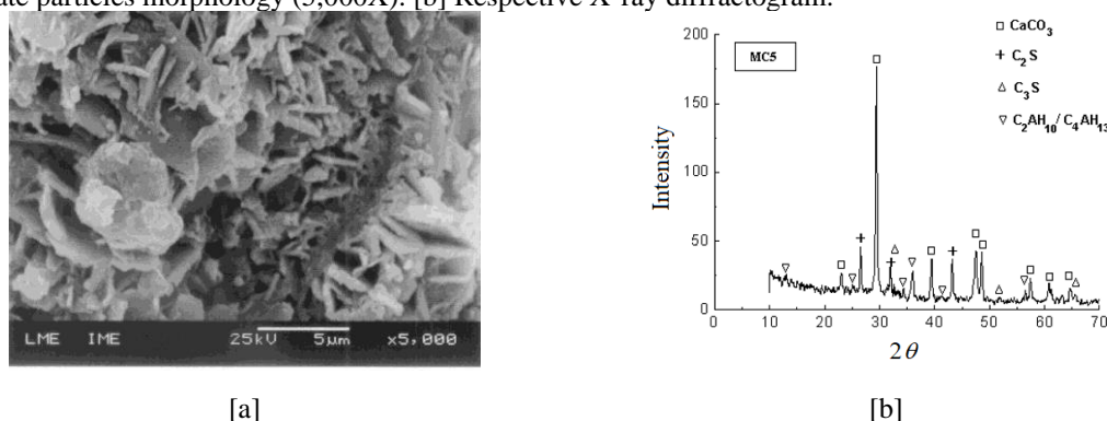
Figure 8. [a] Micrograph (SEM) of the paste with 25% MK and 7.5% Na 2 O (MC5) at 28 days of age. Details of hydrated calcium silico-aluminate particles morphology (5,000X). [b] Respective X-ray diffractogram.
