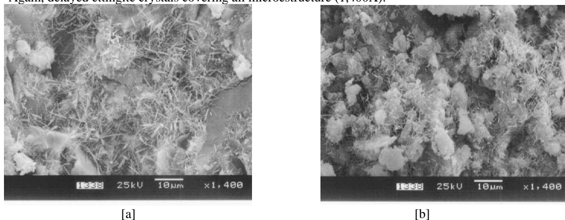
Figure 14. Micrographs (SEM) of the pastes containing: [a] 20% MK and 5% \text{Na}_2\text{SiO}_3 (20MSS). [b] 20% MK and 5% \text{Na}_2\text{SiO}_3 (20MSS) – Again, delayed ettringite crystals covering all microstructure (1,400X).
