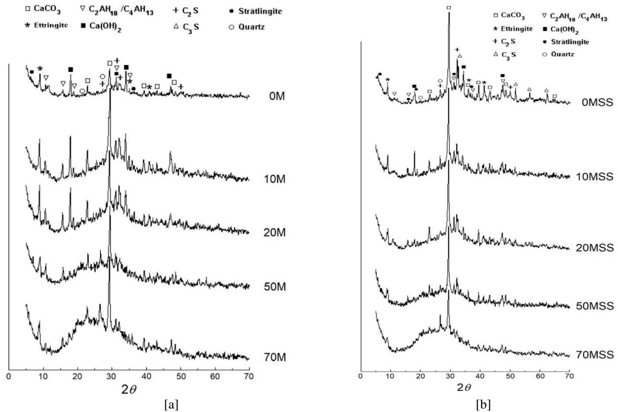
Figure 18. X-ray diffractograms of samples, containing: [a] 0 to 70% MK (not activated); [b] 0 to 70% MK and activated with 5% \text{Na}_2\text{SiO}_3 .
