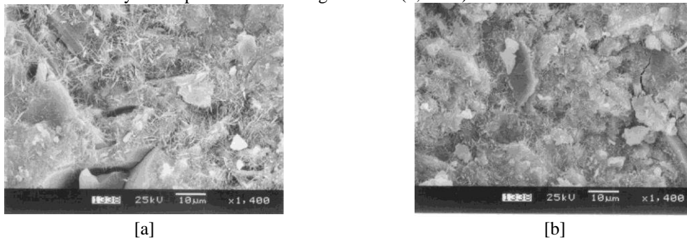
Figure 12. Micrographs (SEM) of the pastes containing: [a] 10% MK (10M). [b] 10% MK and 5% \text{Na}_2\text{SiO}_3 (10MSS) – Both showing formation of massive hydrated products and ettringite fibrils (1,400X).
