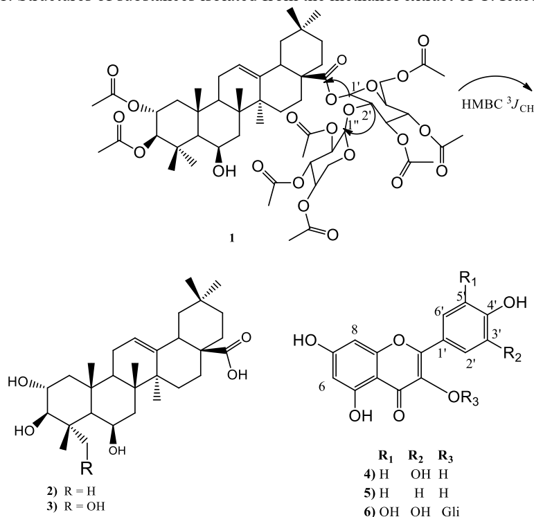
Figure 1. Structures of substances isolated from the methanol extract of C. Icaico leaves.
