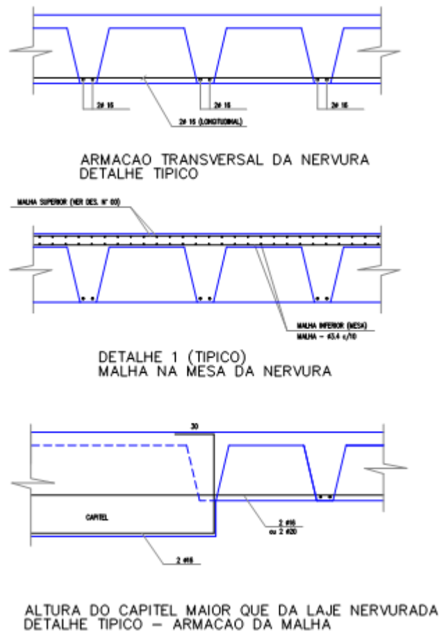
Figure 7 – Detailing of the reinforcements of the ribs
