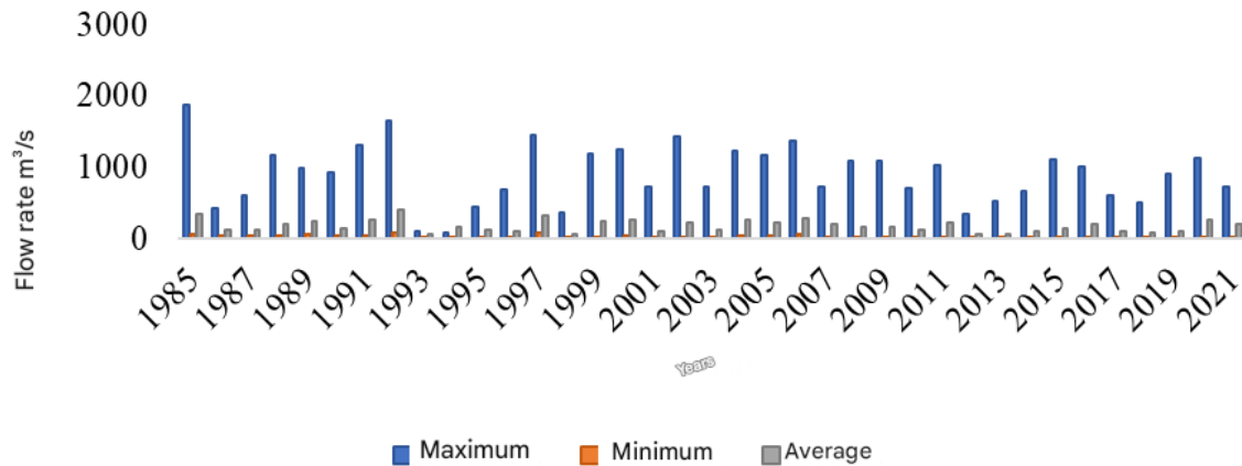
Figure 8. Representative graph of flow in the 51120000 contribution basin.
